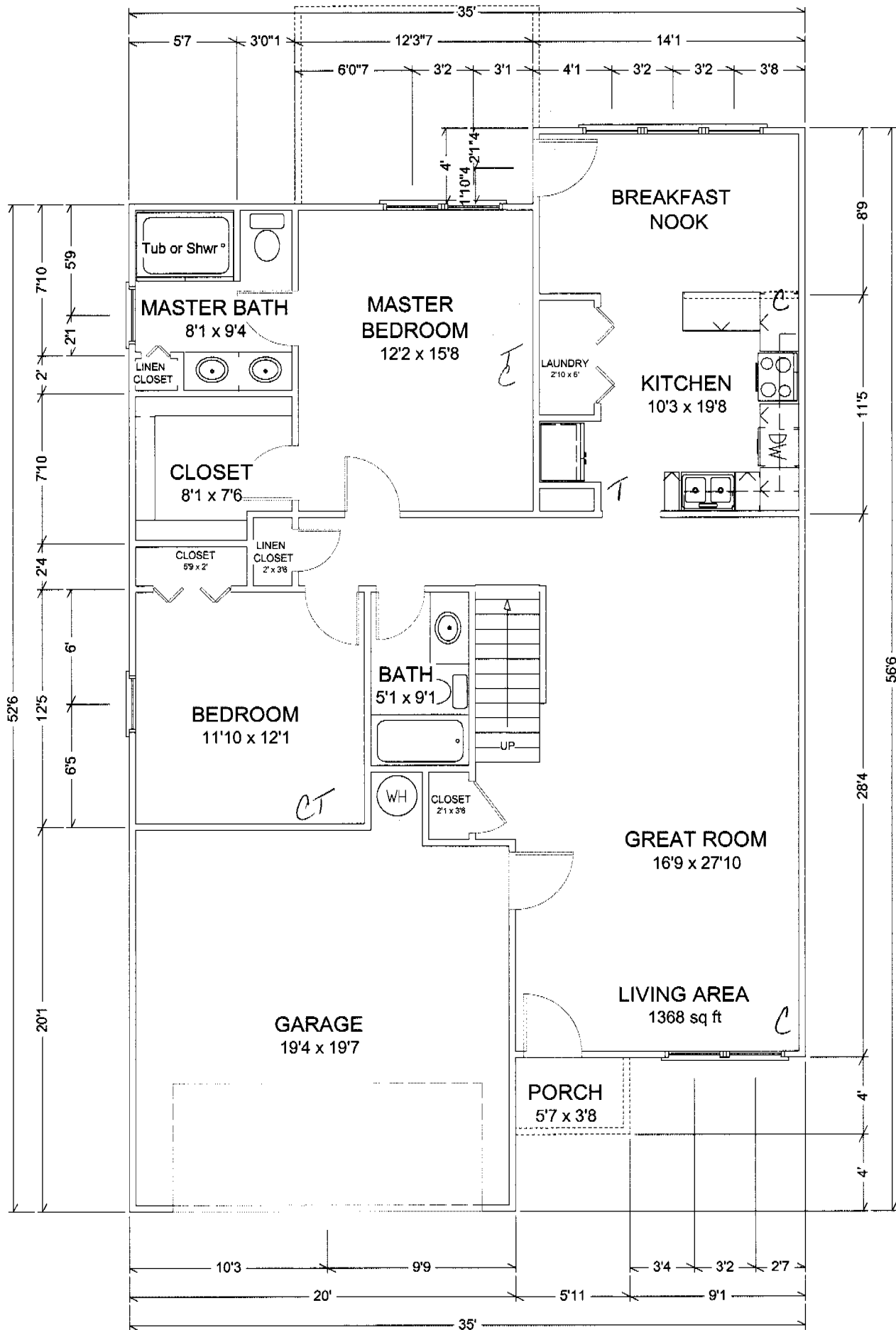
Slate Creek Commons Slab Unit w/Optional Upstairs
